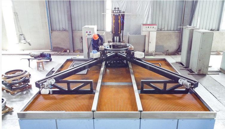
Large - scale slewing bearing quenching
